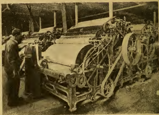
WORSTED CARDING
